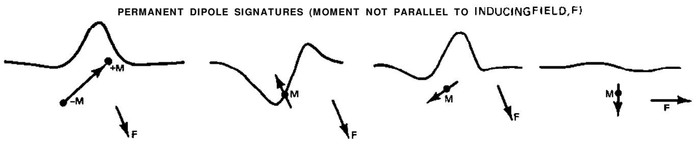
Figure 43. Total Intensity Signatures at Various Inclinations of the Field and for induced or Permanent Magnetic Moments
