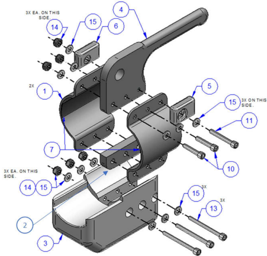
ASSY EXPLODED VIEW
