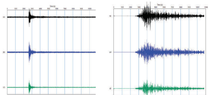
Teleseismic records of M7.7 earthquake in the Aleutian Islands acquired with the Atom-3C for earthquake monitoring.
