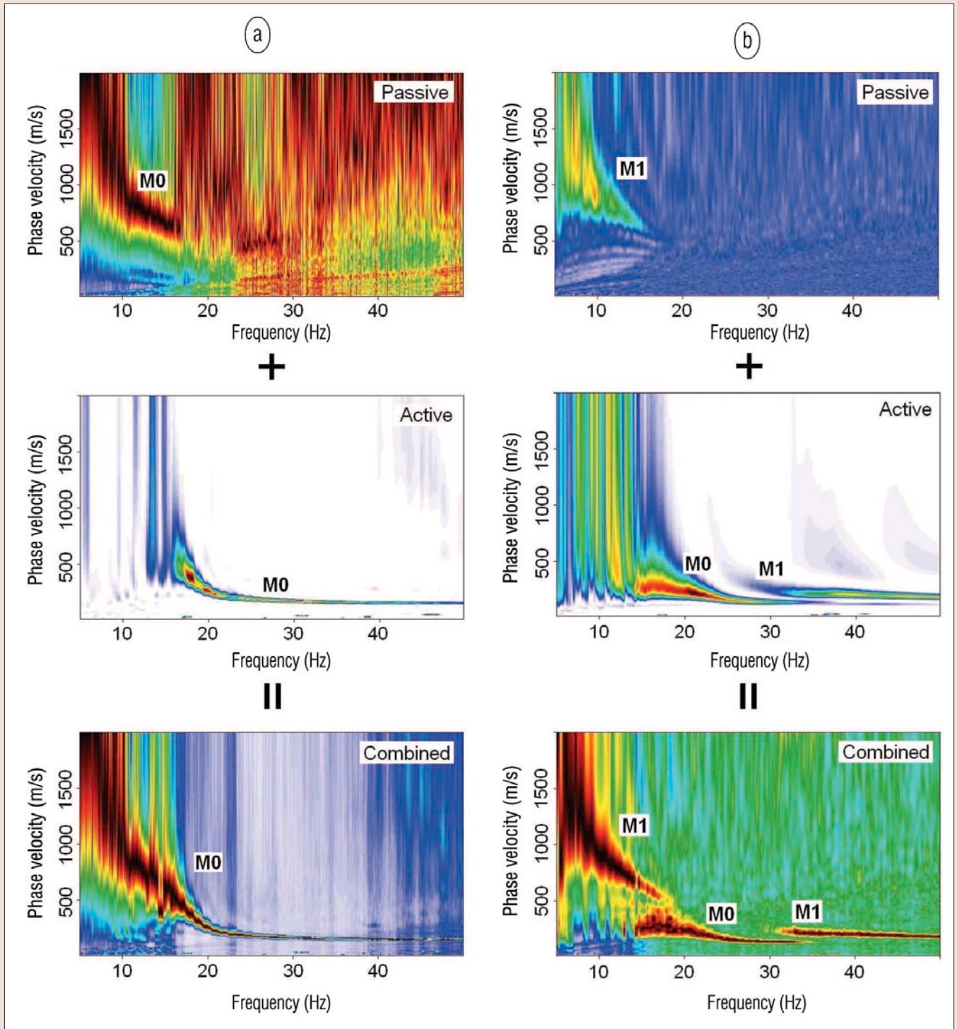
Figure 6. Dispersion images obtained from passive (top) and active (middle) MASW surveys. Two sets of image data are combined to enlarge the frequency range of dispersion (therefore to enlarge the investigation depth range) in (a), whereas in (b) they are combined to help modal identification of recognized dispersion trends and to enlarge the usable bandwidth of dispersion.
