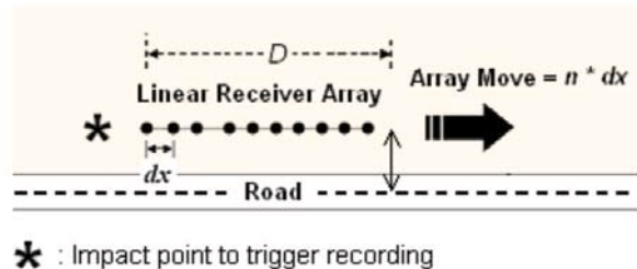
Figure 3. Schematics of data acquisition with passive remote and passive roadside MASW.
