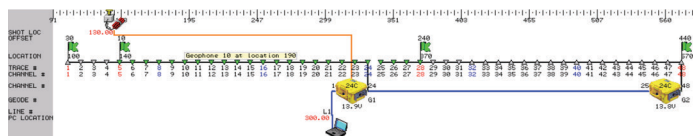
The Geometry Toolbar interactively updates source location, preamp gains, and roll of the line spread.
