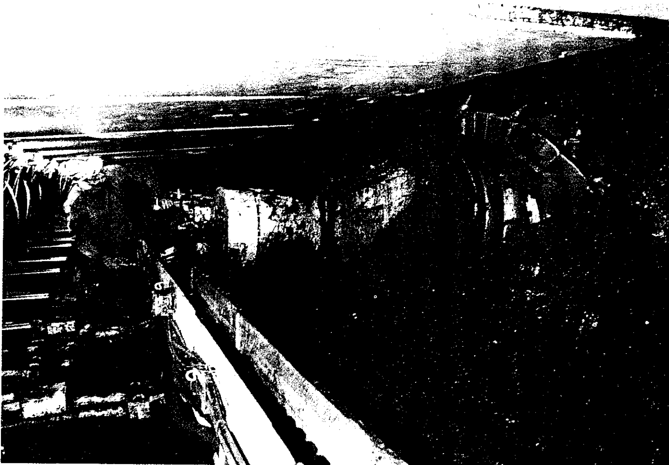
Figure 1. Miner operates the longwall where the shearer cuts the coal while the shields support the roof.
