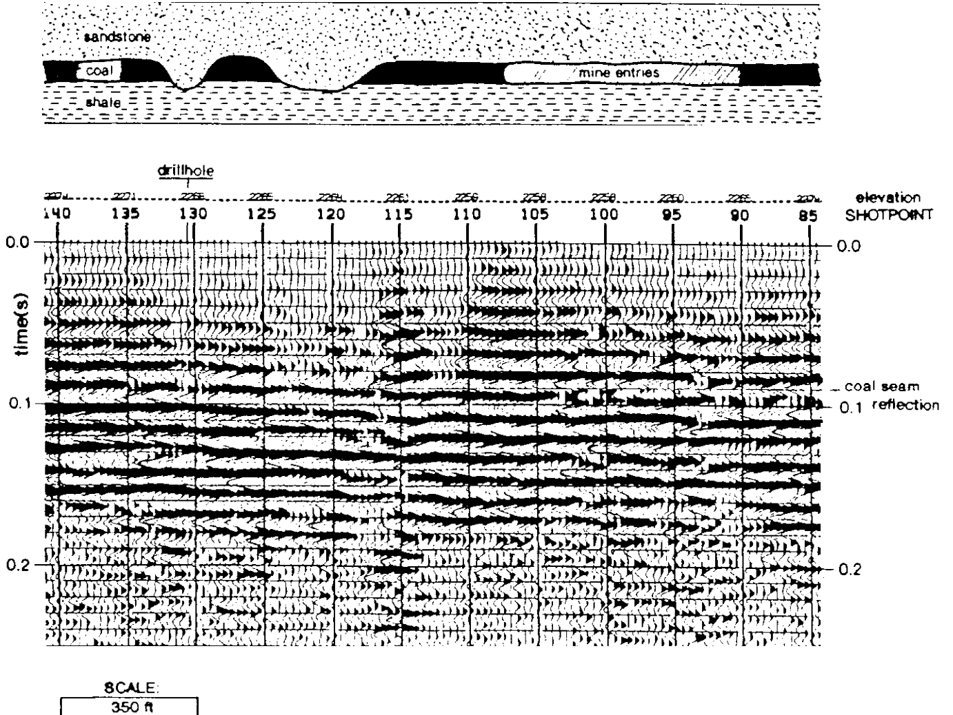
Figure 5. Seismic section of a survey conducted to investigate sandstone washouts.
