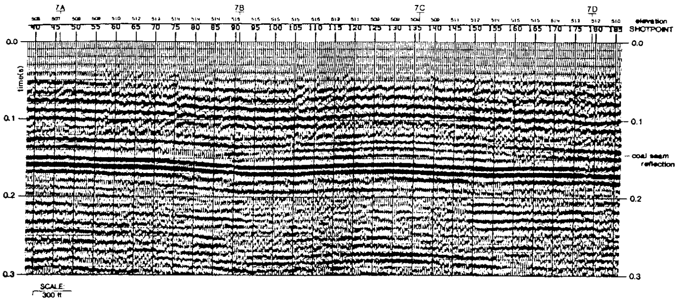
Figure 4. Seismic section of a survey conducted to investigate seam anomalies between
