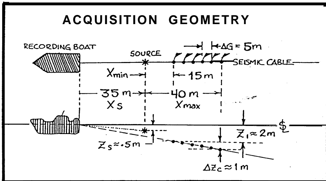
Fig_ 7 - Typical recording configuration, 1987 survey
