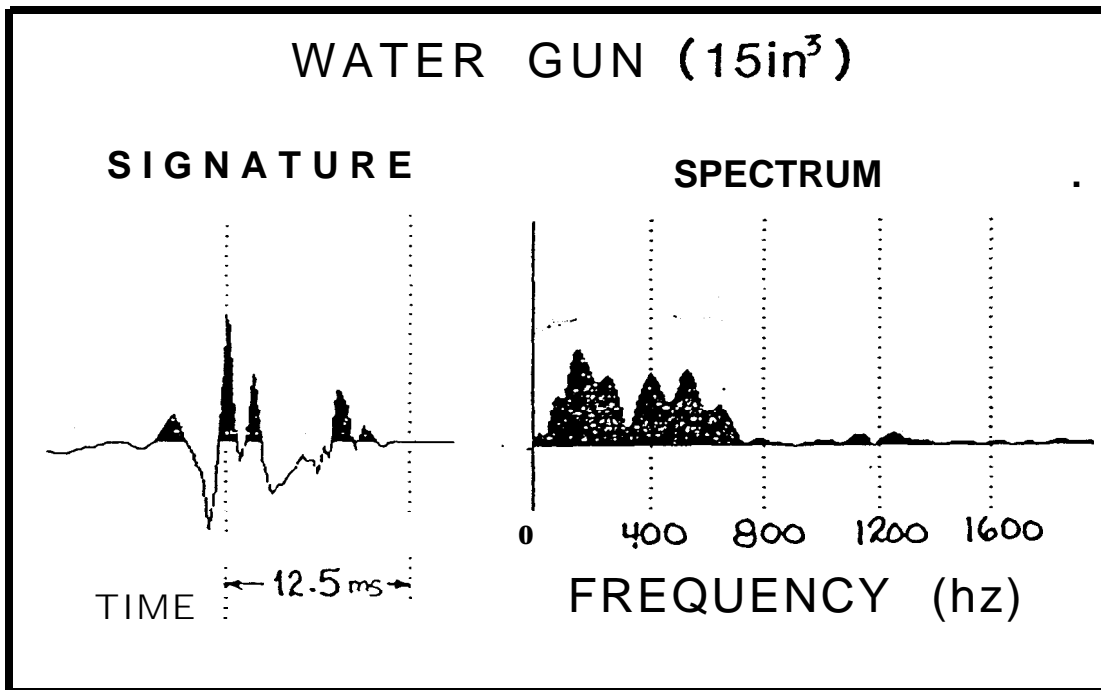
Fig 4 - Watergun signature and spectrum. Phase the culprit.
