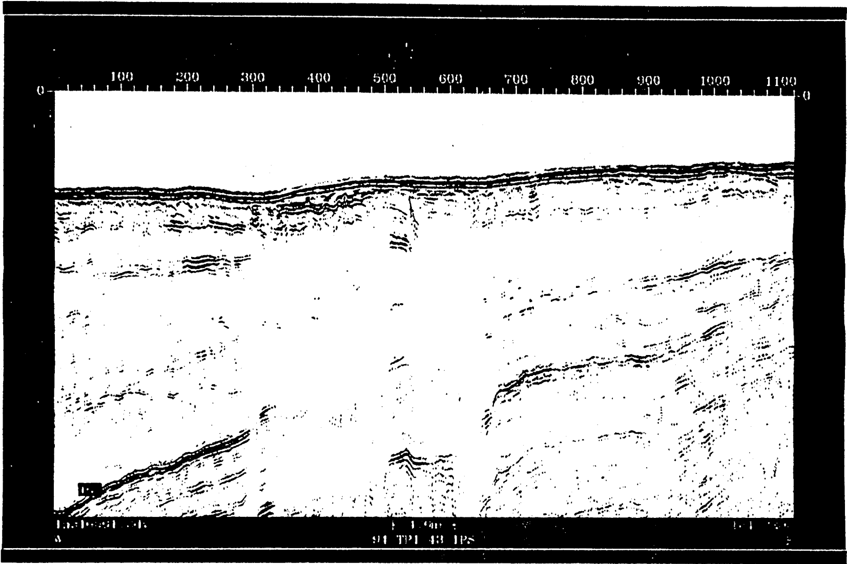
Fig. 12 - Line 3181. Processed data.
