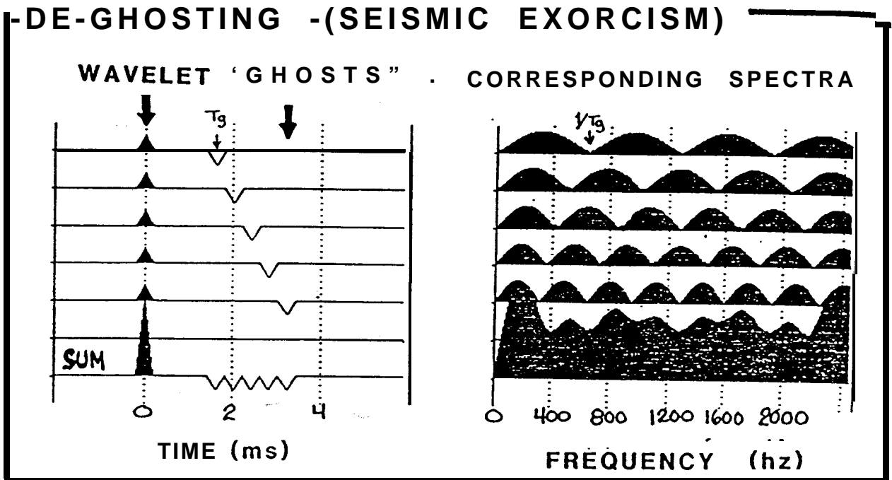
Fig. 6 - Summing the wevelets with varying ghost times, T_g , spreads the notches and facilitates deconvolution
