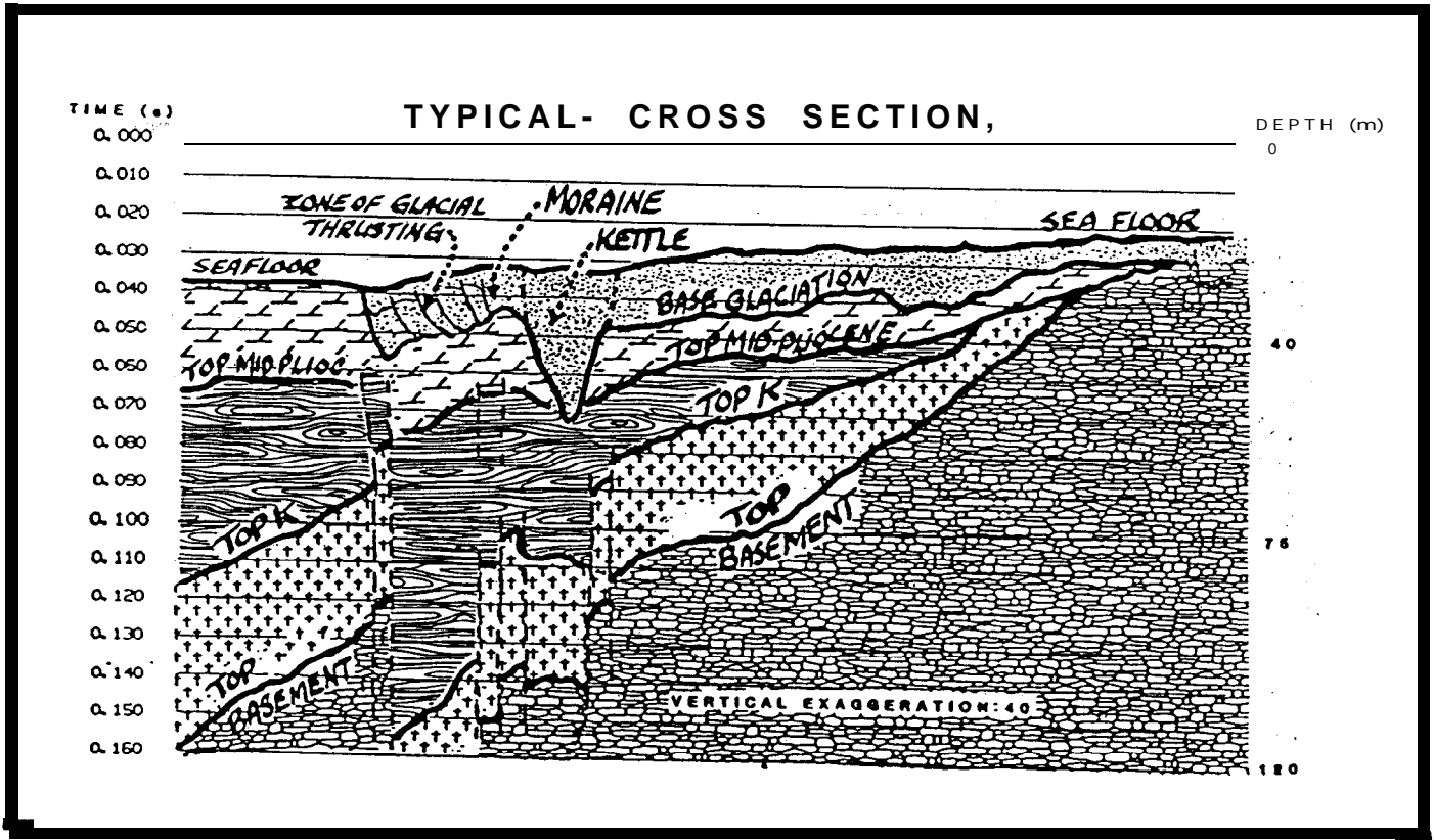
Fig_ 2 - Typical cross section based on interpretation of line 3181
