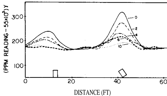
Fig. 5. Magnetometer scans over pattern 1. Labels on curves indicate traverses with offset in feet. Measurements were made on a 2 x 2 ft grid, but some of the scans have been omitted for the sake of clarity in this and subsequent figures.
