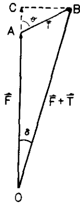
Fig. 3. Effect of an anomaly of magnetic field, \vec{T} , on the earth's magnetic field, \vec{F}
