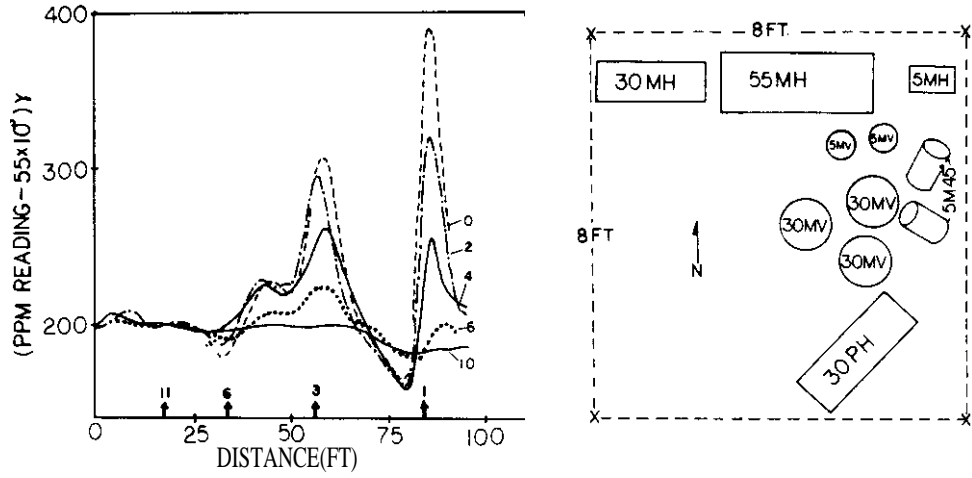
Fig. 8. Magnetometer scans over pattern 4. Actual position of drums is indicated by arrows labeled with depth of burial. Labels on curves indicate traverses with offset in feet.
