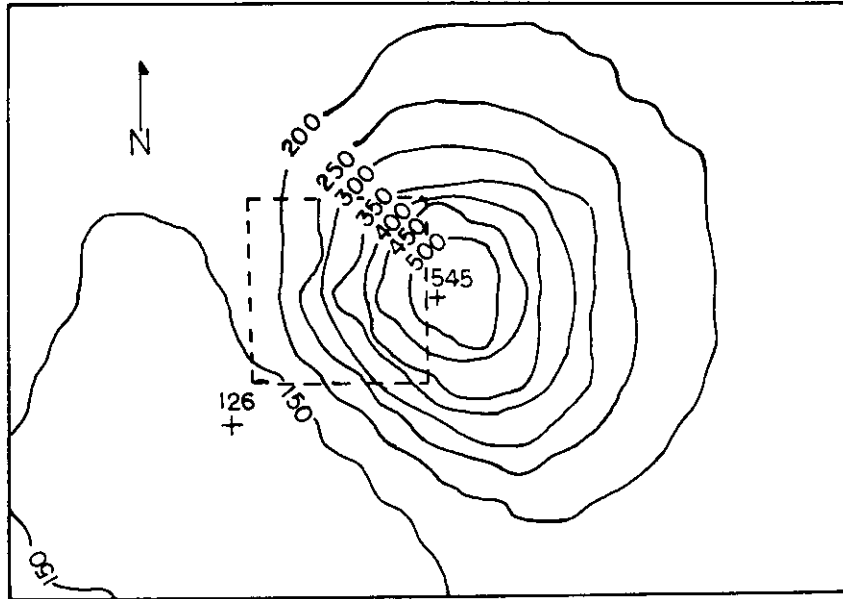
Fig. 10. Magnetic field contour map of the "trash dump" using the PPM. The actual magnetic field is 55 \times 10^3 y plus the contour magnetic field label in units of y . The "trash dump" boundary is indicated by the dashed lines.
