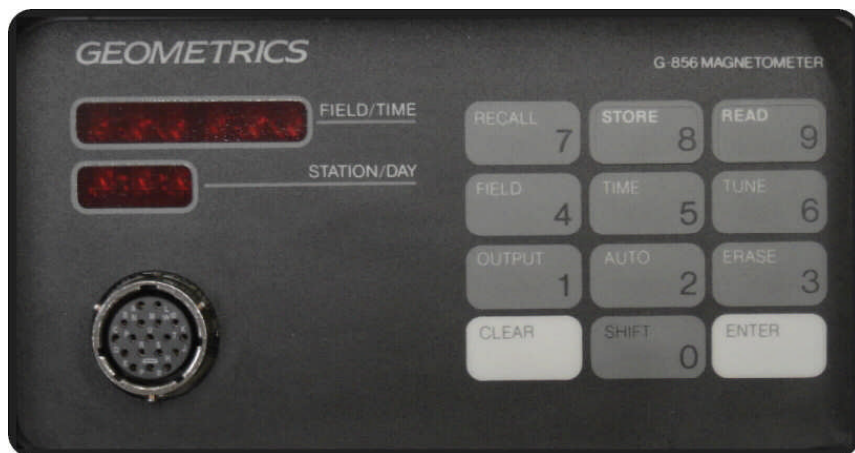
Figure 19. G-856AX console display and keypad.
